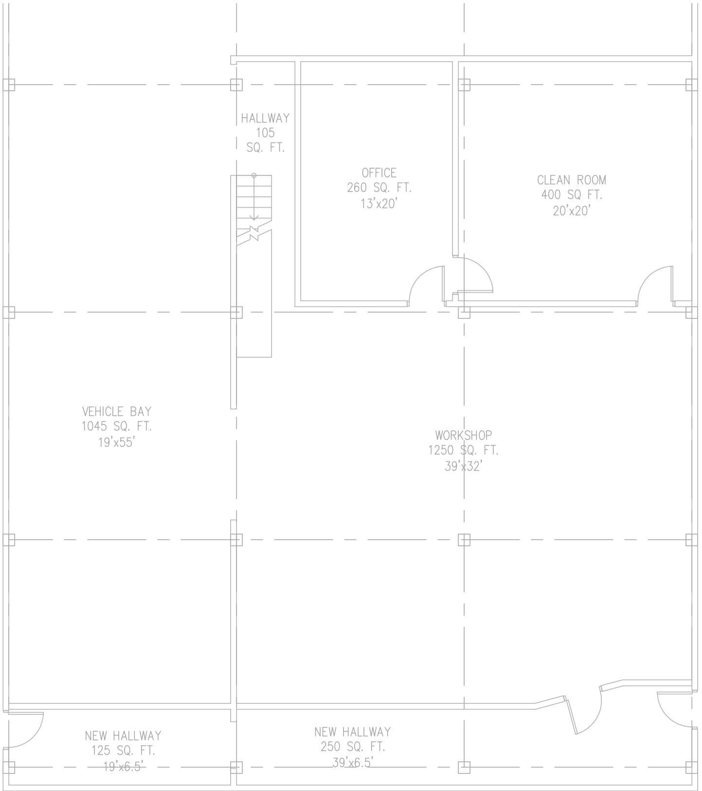
1 FLOOR PLAN 1/8" = 1'-0"
